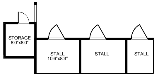
BARN 340 SQ.FT
